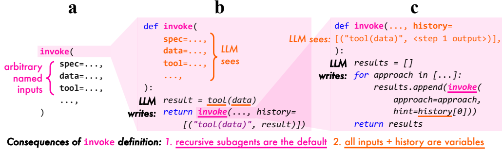
Figure 2: In the functional version of invoke , the LLM writes a complete implementation for every invocation. A closed agent loop arises from tail-recursive invoke .
